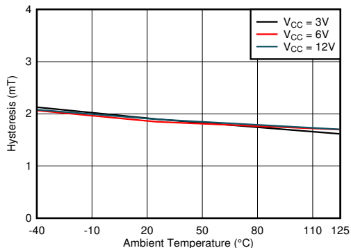
图 7-5. Hysteresis vs Temperature
