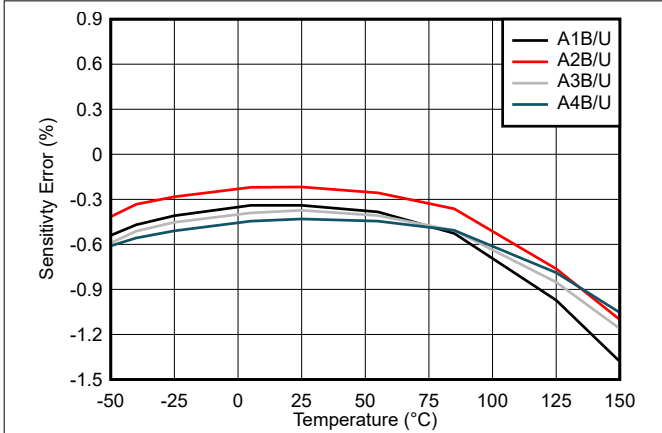
图 7-1. TMCS1108 Sensitivity Error vs. Temperature
