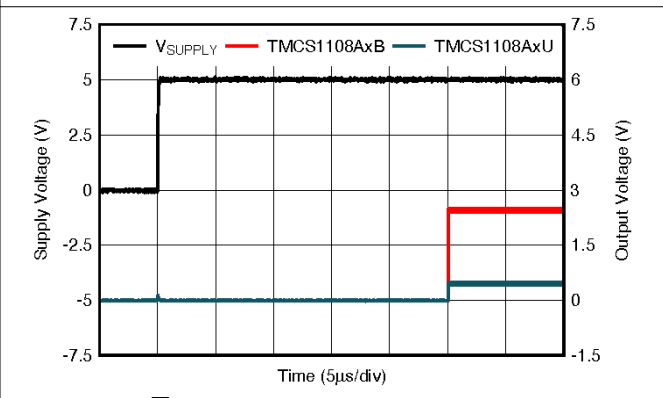
图 7-12. Startup Transient Response
