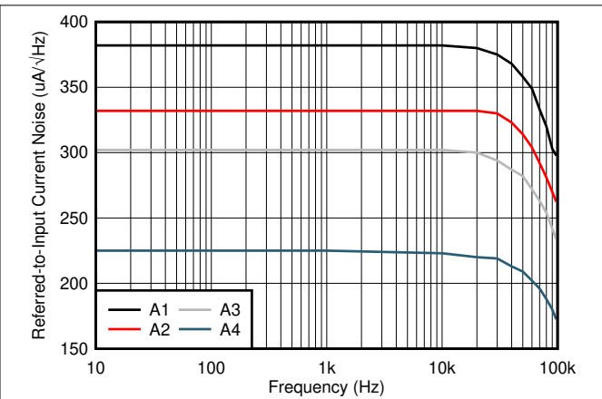
图 7-8. Input-Referred Noise vs. Frequency
