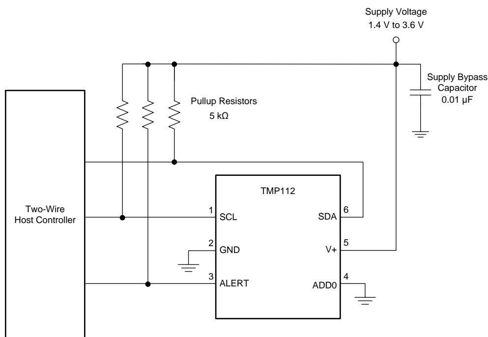
Figure 17. Typical Connections
