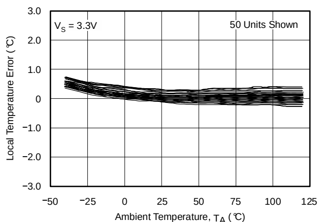
Figure 20. Local Temperature Error vs TMP411 Ambient Temperature
