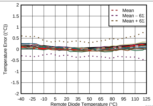
Figure 20. TMP451-Q1 Remote Diode Temperature Drift (Diode-Connected 2N3906)
