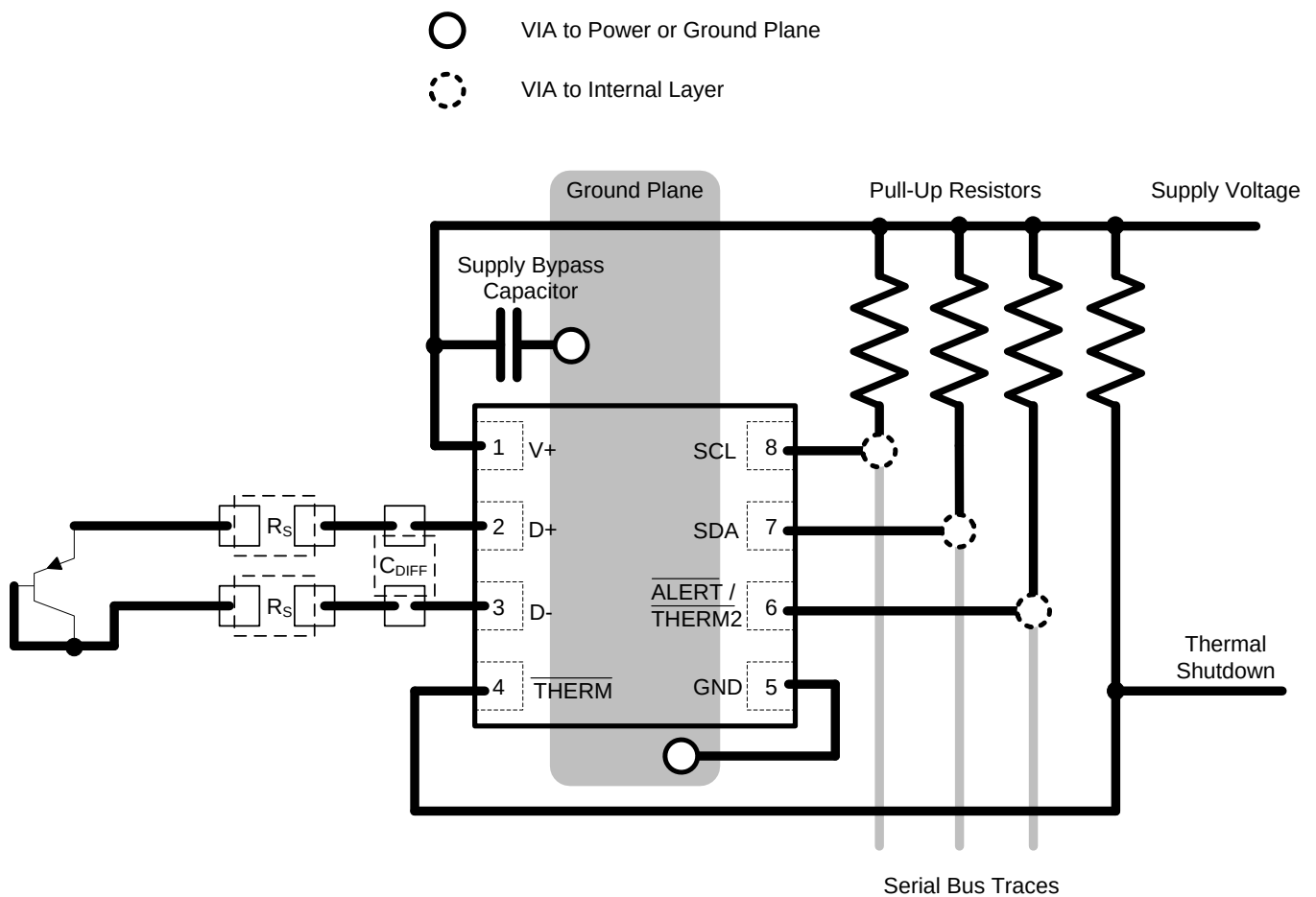
Figure 23. TMP451-Q1 Layout Example
