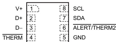
Pin Functions
