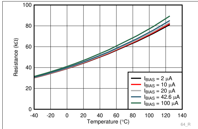
图 1. Resistance vs. Ambient Temperature Using Multiple Bias Currents
