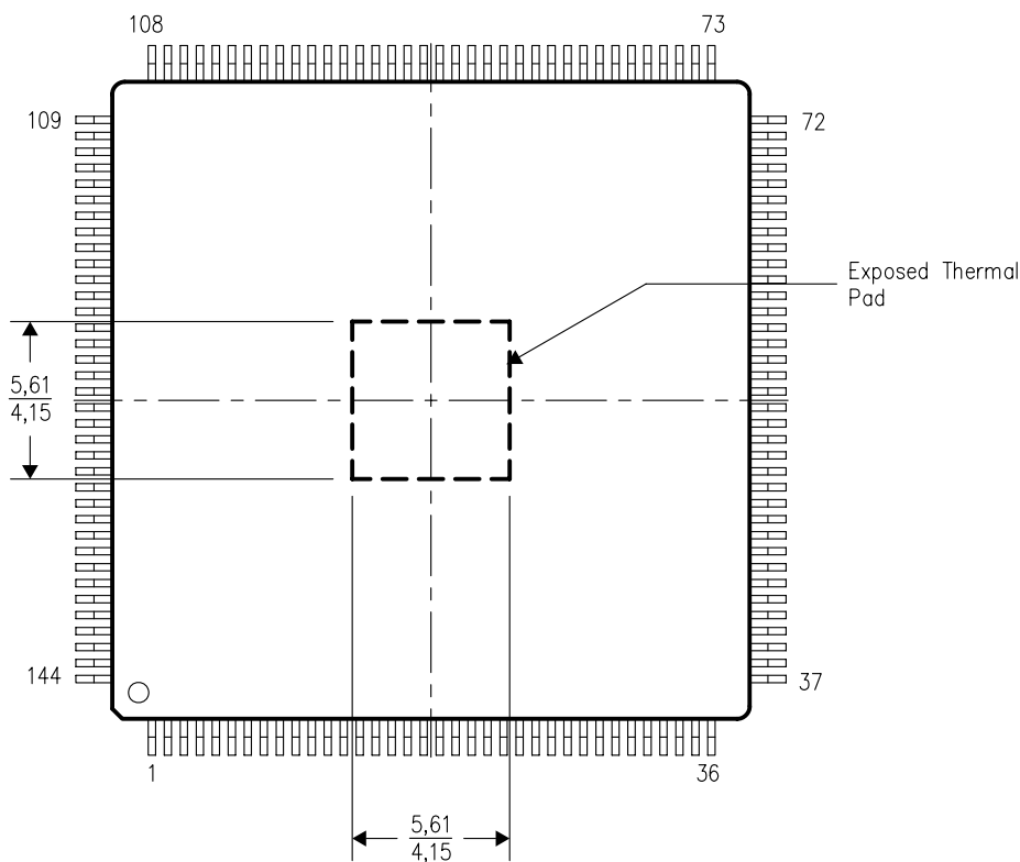
Top View
