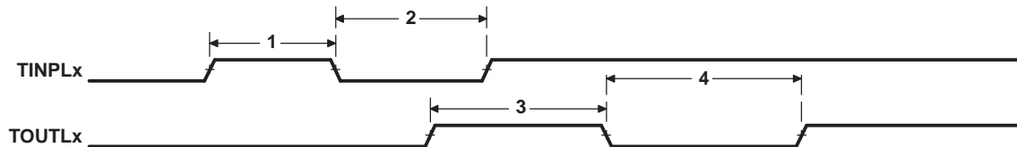
Figure 7-73. Timer Timing
