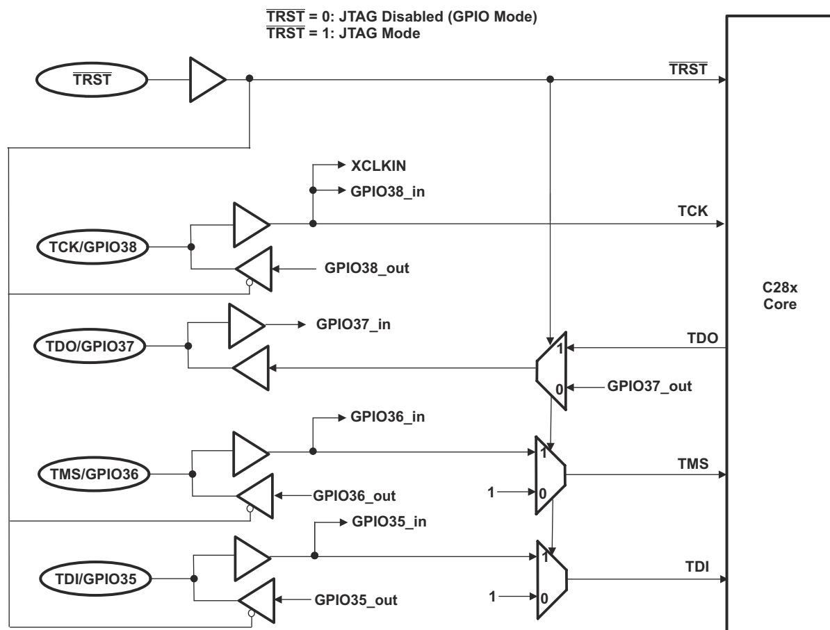
图 8-44. JTAG/GPIO Multiplexing
