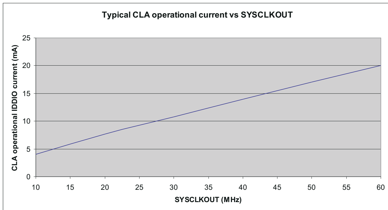
图 7-3. Typical CLA Operational Current Versus SYSCLKOUT
