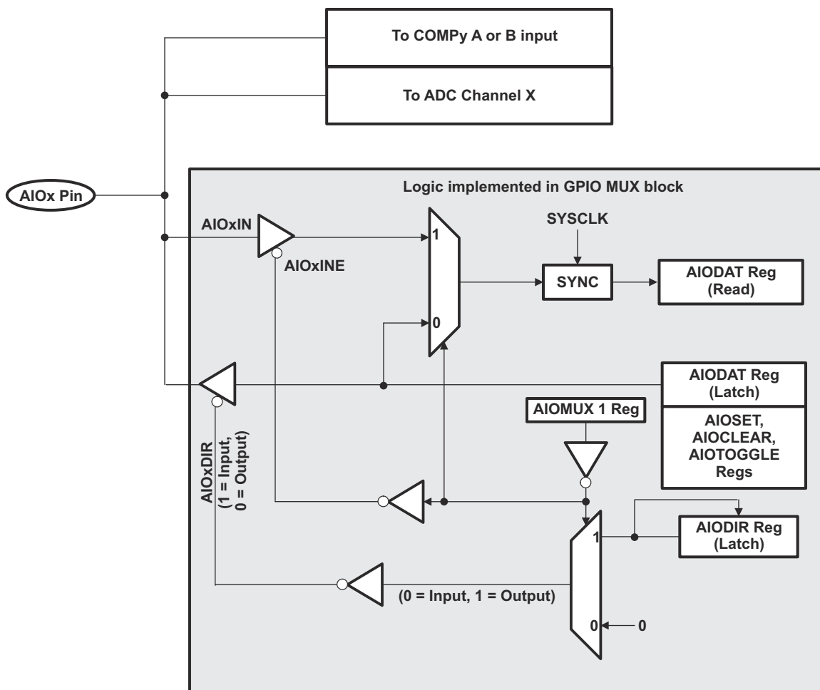
图 8-25. AlOx Pin Multiplexing
