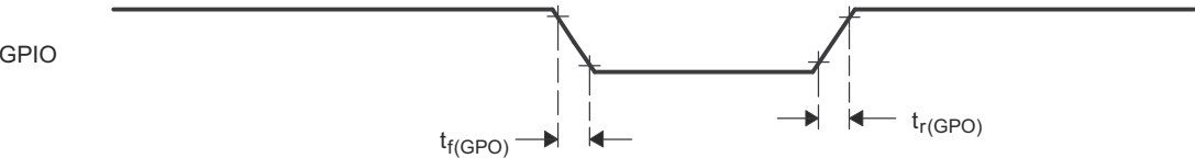
图 8-46. General-Purpose Output Timing
