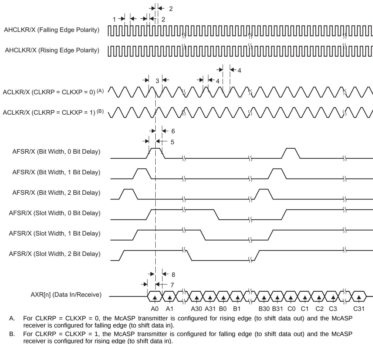
Figure 6-49. McASP Input Timing
