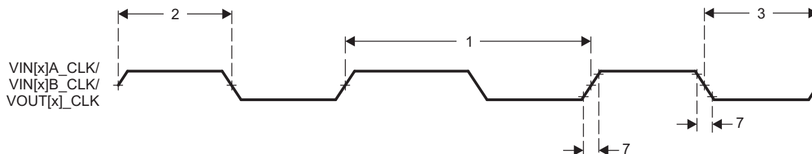
Figure 8-68. HDVPSS Clock Timing
