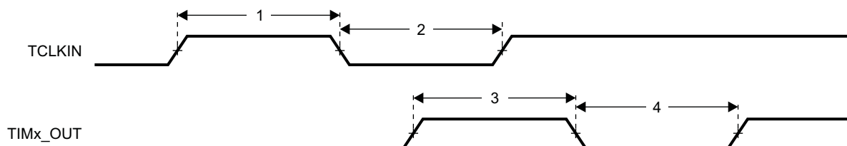
Figure 8-88. Timer Timing
