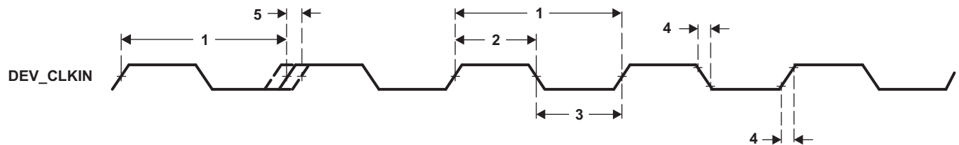
Figure 7-6. DEV_CLKIN Timing
