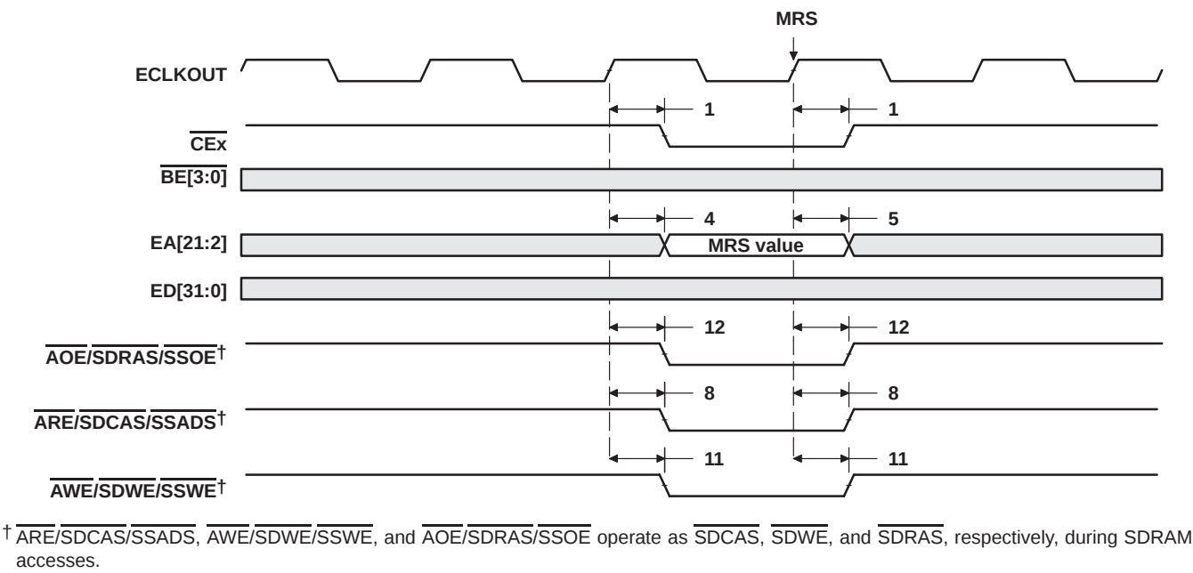
Figure 37. SDRAM MRS Command
