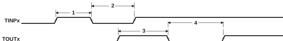
Figure 52. Timer Timing
