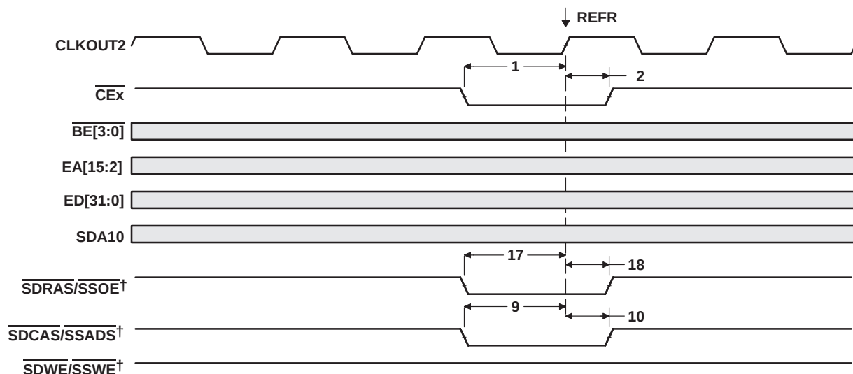
Figure 25. SDRAM REF Command
