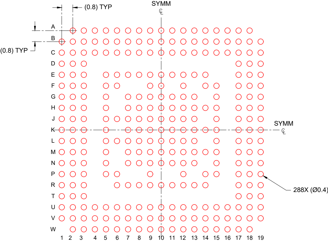
SOLDER PASTE EXAMPLE BASED ON 0.150 mm THICK STENCIL SCALE: 6X
