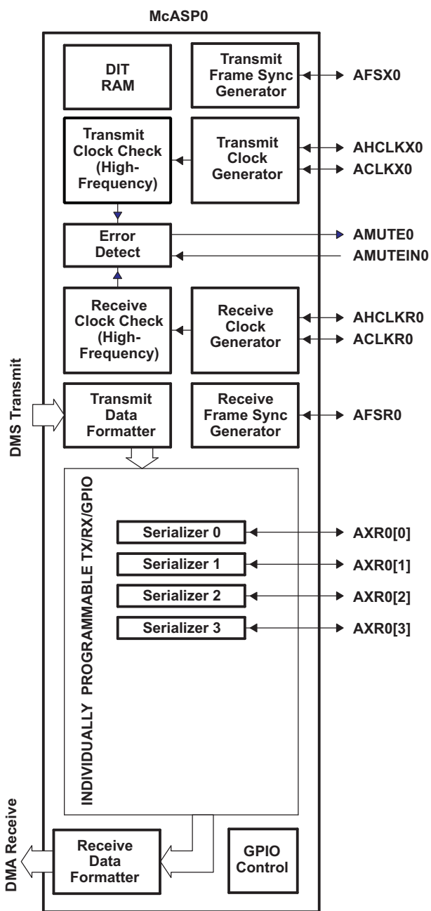
Figure 6-36. McASP0 Configuration
