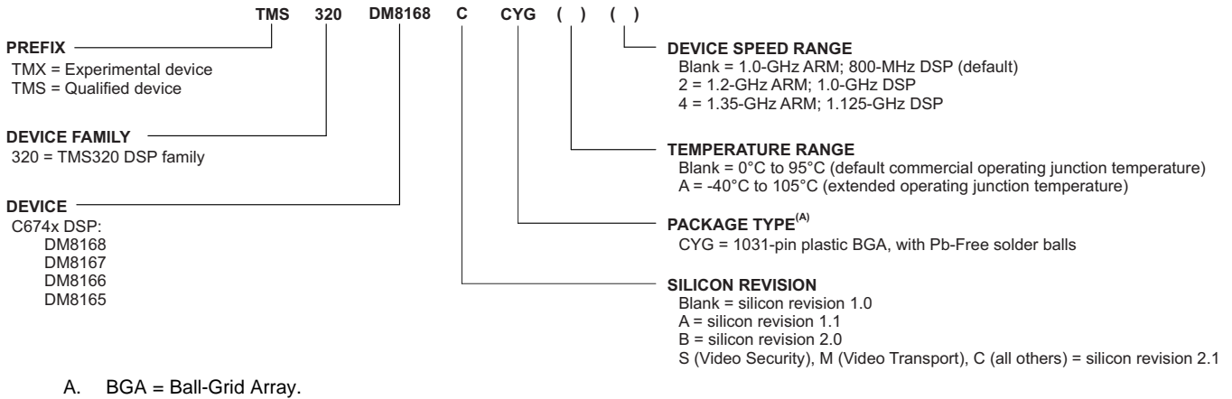
Figure 9-1. Device Nomenclature
