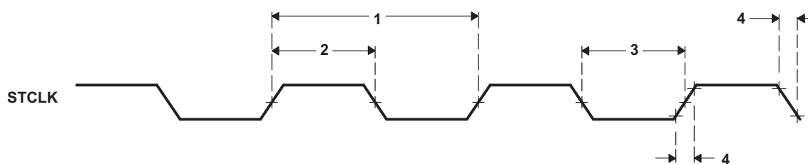
Figure 6-32. STCLK Timing
