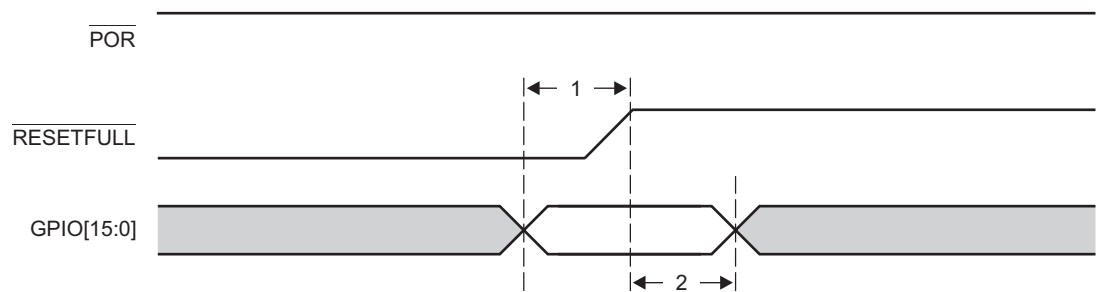
Figure 7-6 Boot Configuration Timing
