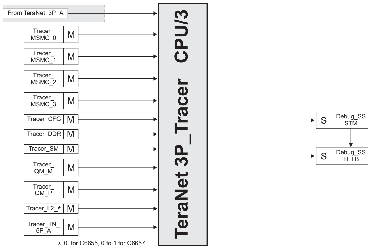
Figure 4-4 TeraNet 3P_Tracer
