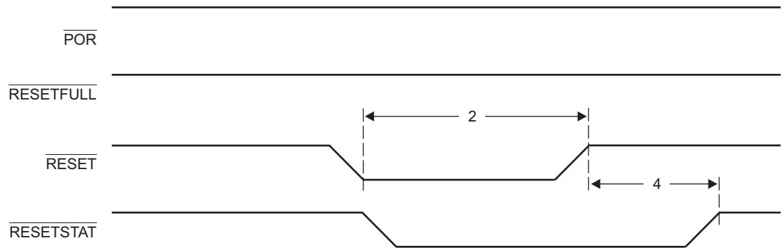
Figure 7-5 Soft/Hard-Reset Timing
