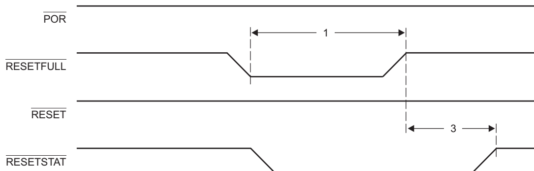
Figure 7-4 RESETFULL Reset Timing
