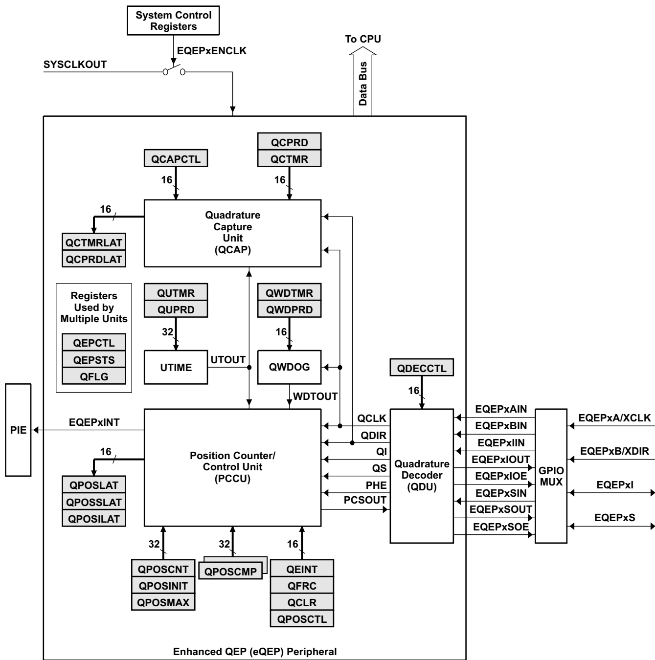
图 8-53. eQEP Functional Block Diagram
