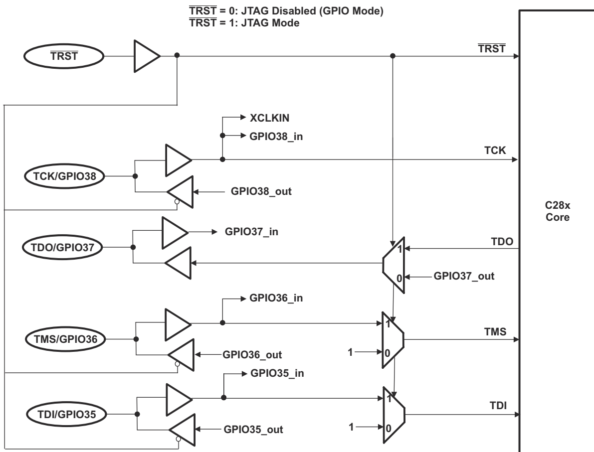
图 8-54. JTAG/GPIO Multiplexing
