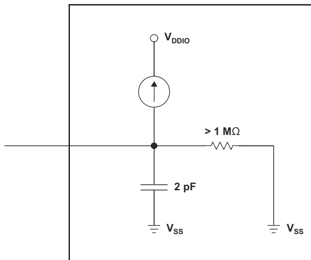
图 8-59. Input Resistance Model for a GPIO Pin With an Internal Pullup
