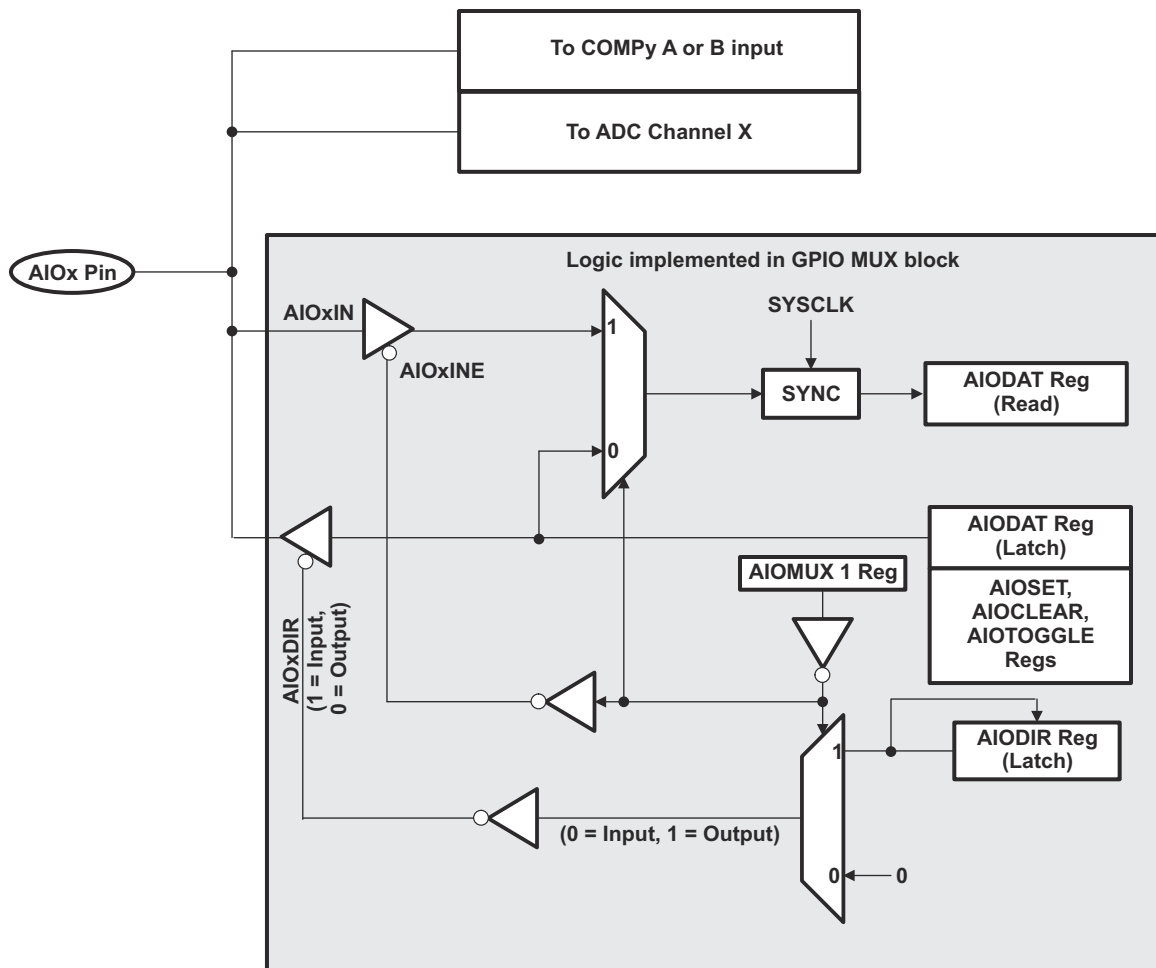
图 8-29. AlOx Pin Multiplexing
