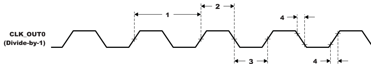
Figure 6-13. CLKOUT0 Timing
