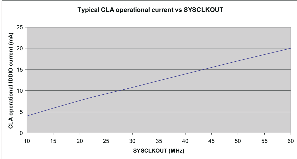
图 7-3. Typical CLA Operational Current Versus SYSCLKOUT
