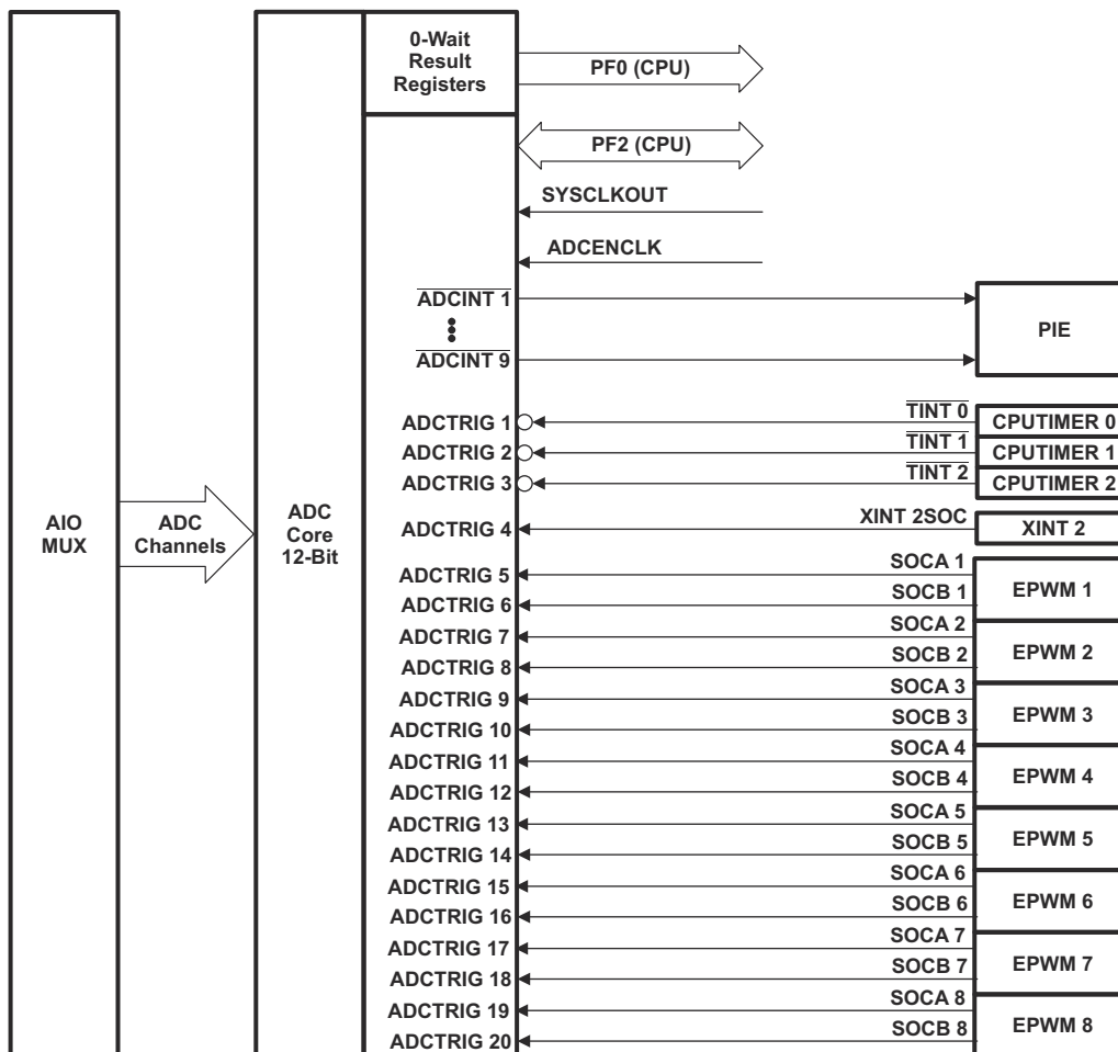
图 8-21. ADC Connections
