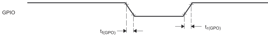
图 8-46. General-Purpose Output Timing
