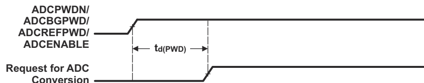
图 8-23. ADC Conversion Timing
