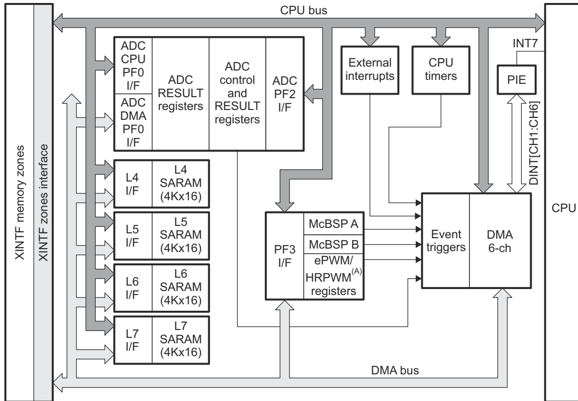
图 8-1. DMA Functional Block Diagram
