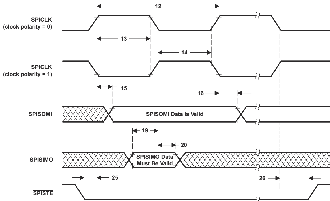
图 7-19. SPI Slave Mode External Timing (Clock Phase = 0)
