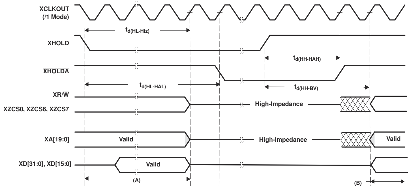
图 7-35. External Interface Hold Waveform
