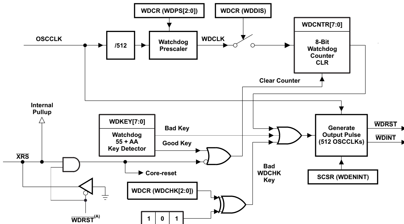
Figure 6-22. Watchdog Module
