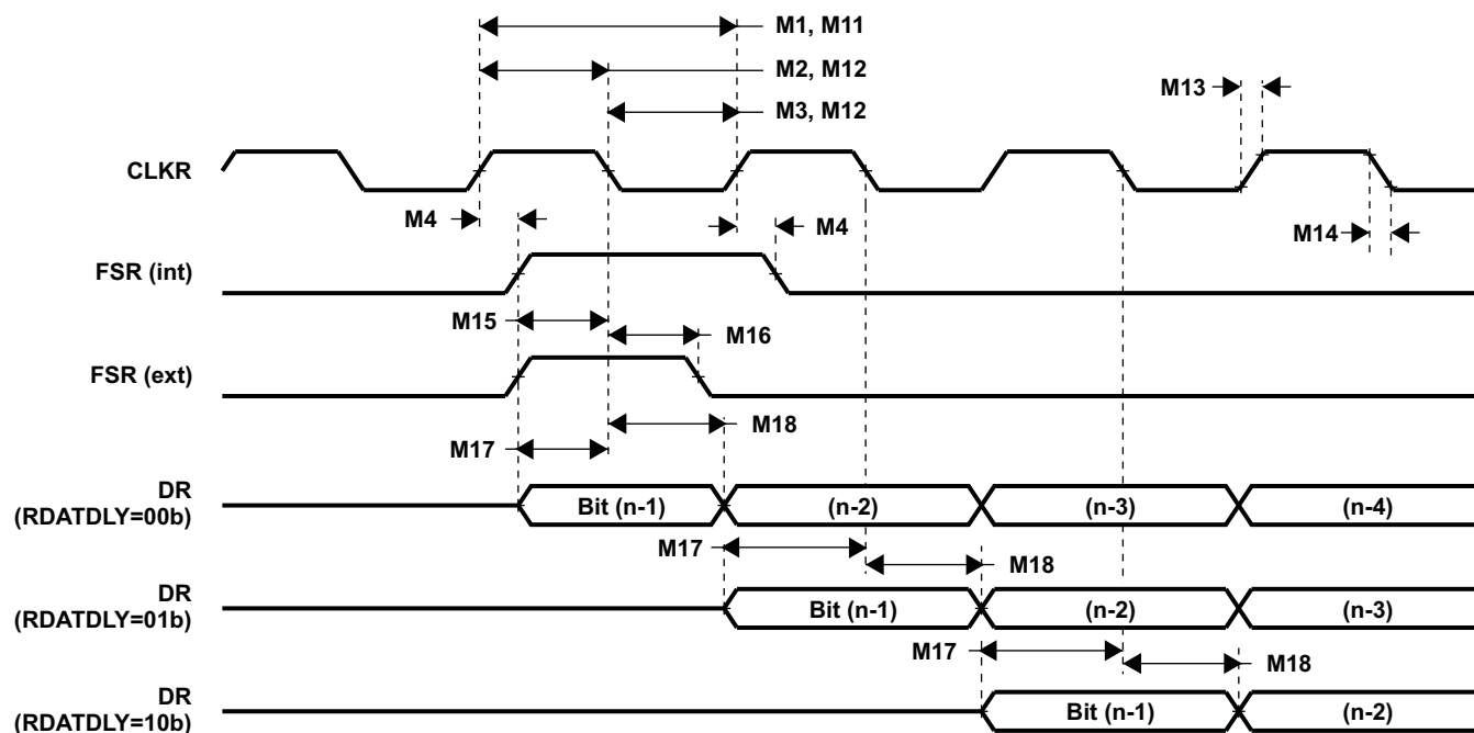
Figure 5-39. McBSP Receive Timing
