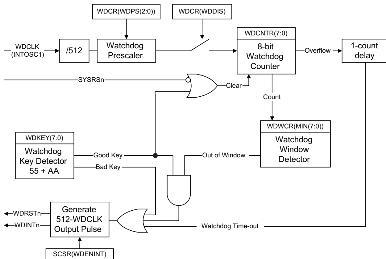
图 6-5. Windowed Watchdog
