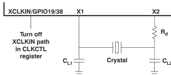
图 8-8. Using the On-chip Crystal Oscillator
