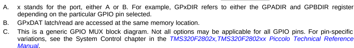
Figure 6-40. GPIO Multiplexing
