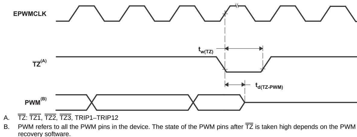
Figure 5-52. PWM Hi-Z Characteristics
