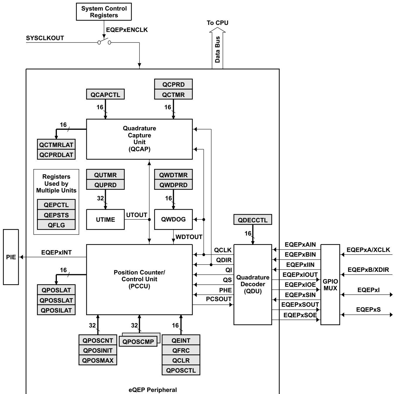
图 8-43. eQEP Functional Block Diagram
