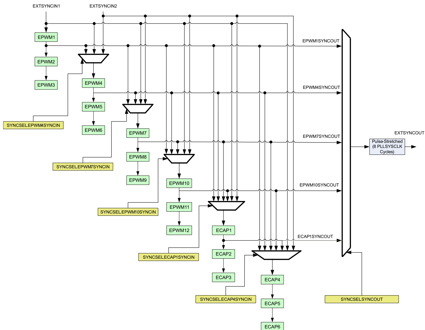
图 5-47. Synchronization Chain Architecture
