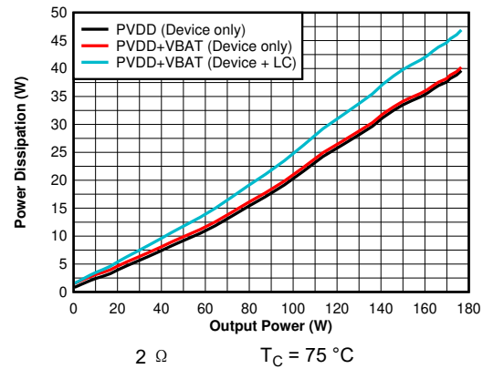
图 6-46. Power Dissipation vs Output Power - 2 \Omega
