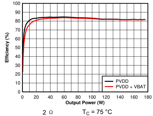
图 6-44. Efficiency vs Output Power - 2 \Omega
