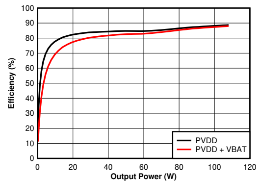
图 6-5. Efficiency vs Output Power - 4 \Omega
