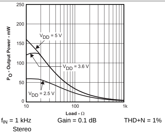
Figure 28. Output Power vs Load
