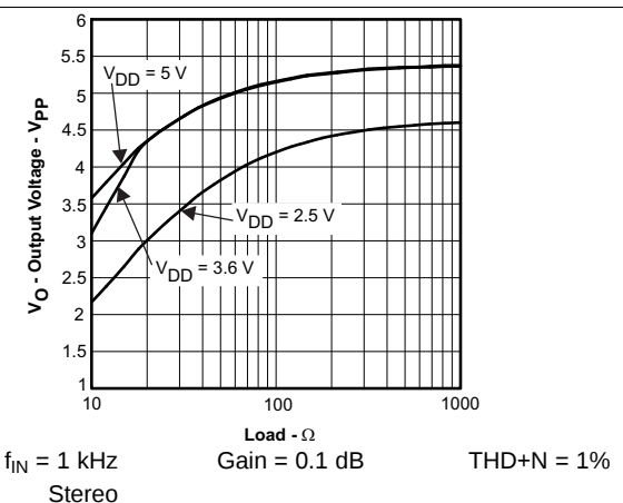
Figure 30. Output Voltage vs Load
