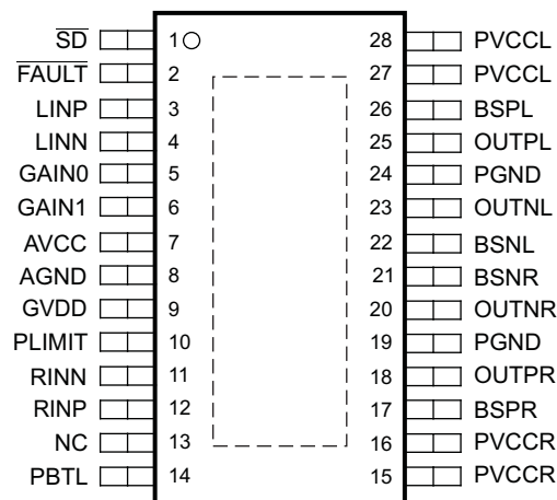
PWP Package 28-Pin HTSSOP With PowerPAD™ Top View
