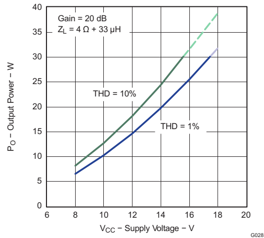
Figure 47. Output Power vs Supply Voltage (PBTl)
