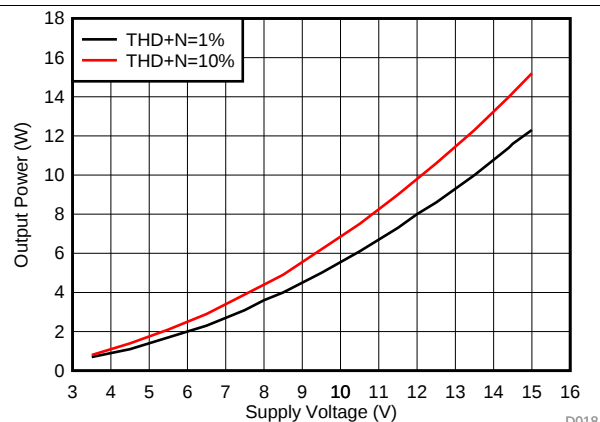
图 8. Output Power vs Supply Voltage (BTL)
