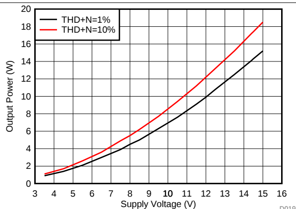
图 7. Output Power vs Supply Voltage (BTL)
