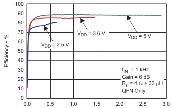
Figure 16. Efficiency vs Output Power (Per Channel)
