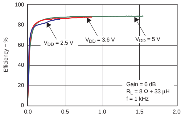
Figure 15. Efficiency vs Output Power (Per Channel)
