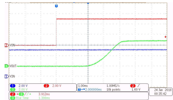
图 7-14. Turn-On at 5 V (CT = 1000 pF)
