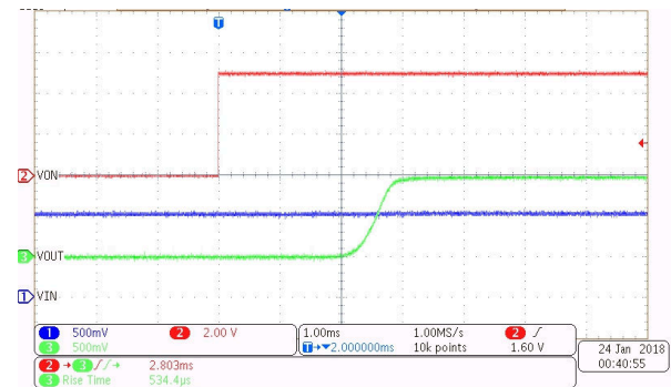
图 7-18. Turn-On at 1 V (CT = 1000 pF)
