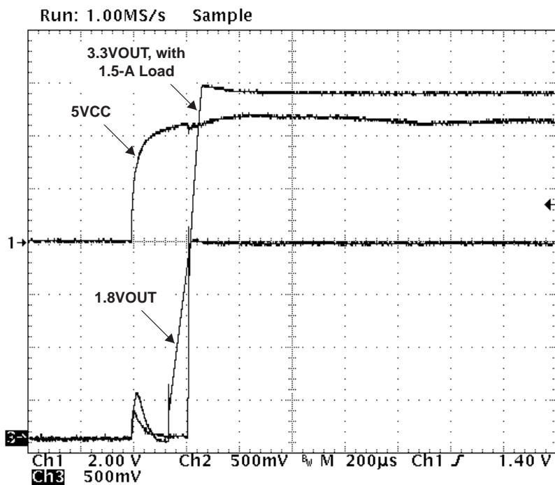
Figure 4. Power-Up Sequence
