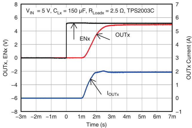
Figure 27. TPS2003C Enable into 2.5 \Omega and 150- \mu F Load
