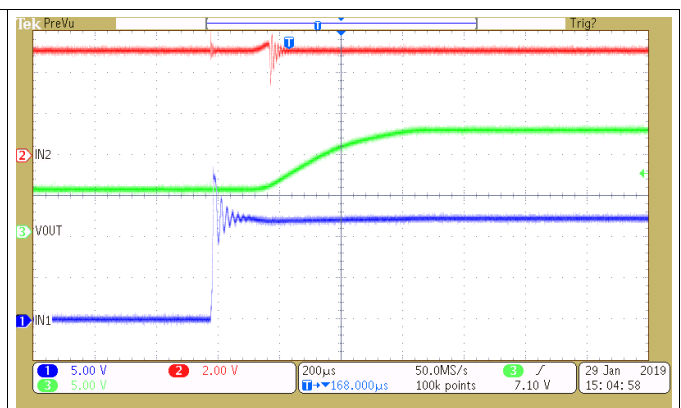
图 41. TPS2121 Hotplug Event with TVS1800
