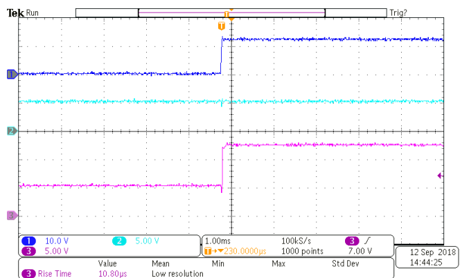
图 30. Automatic Switchover from IN2 to IN1
