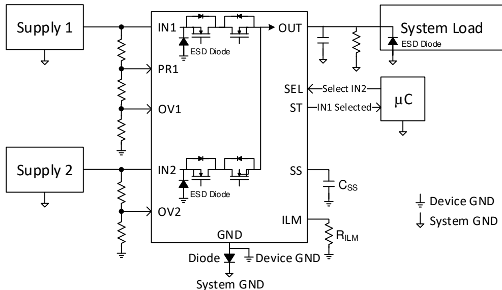
图 38. TPS212x Reverse Polarity Configuration
