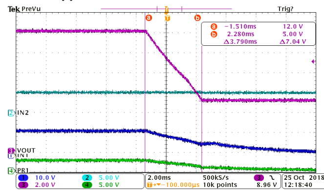
图 29. Automatic Switchover from IN1 to IN2
