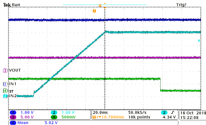
图 35. Switchover from IN1 to IN2
