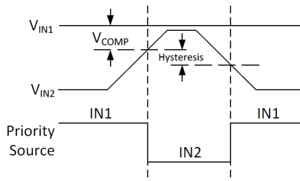
图 19. VCOMP Priority Source Selection
