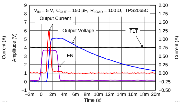
Figure 12. TPS2065C Output Rise / Fall 100Ω
