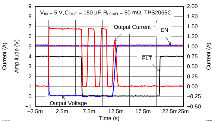
Figure 14. TPS2065C Pulsed Short Applied
