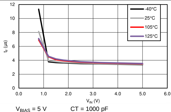
Figure 17. t_F vs V_{IN}
