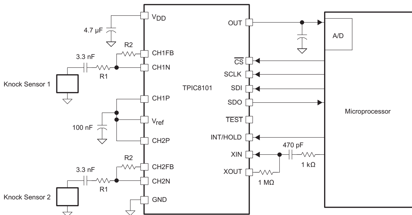
Figure 5. Application Schematic
