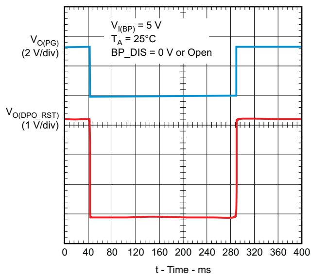
Figure 18. SP to BP Automatic Swicchover Enabled
