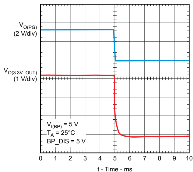
Figure 17. SP to BP Automatic Swicchover Disabled
