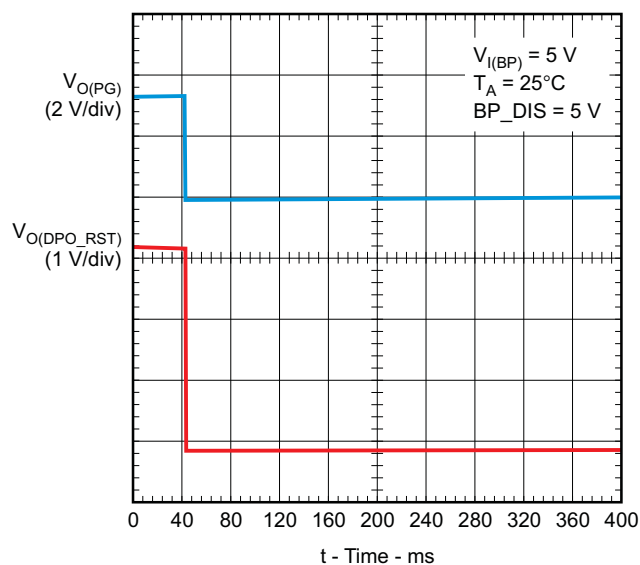
Figure 19. SP to BP Automatic Swicchover Disabled
