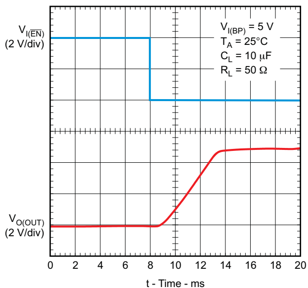
Figure 3. Turnon Delay and Rise Time (BP Switch)
