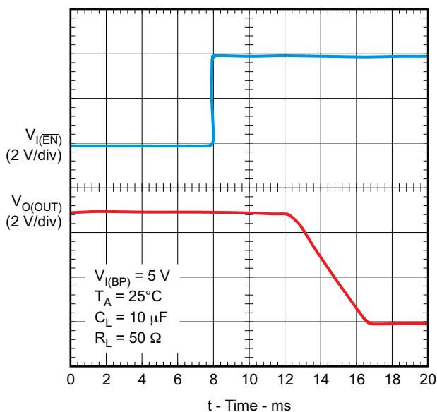
Figure 4. Turnoff Delay and Fall Time (BP Switch)
