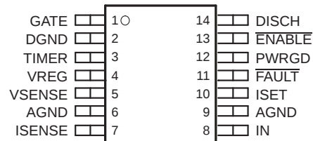
D OR PW PACKAGE (TOP VIEW)
