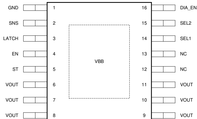
Figure 6-1. PWP Package 16-Pin HTSSOP Top View
