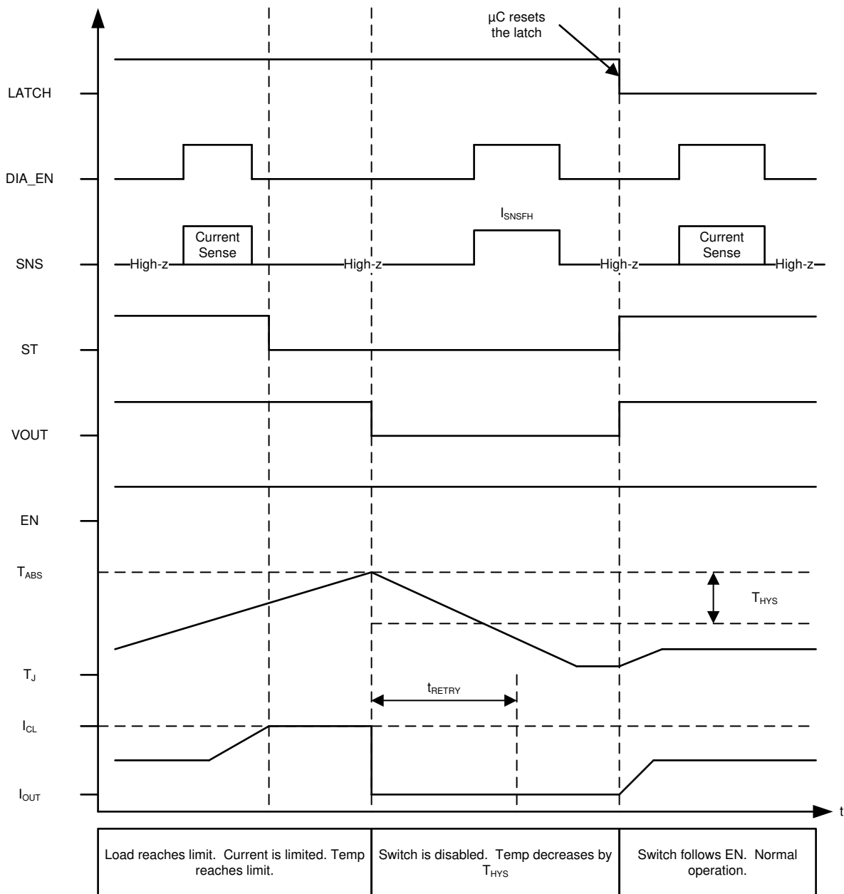
Figure 9-4. Current Limit - Latched Behavior
