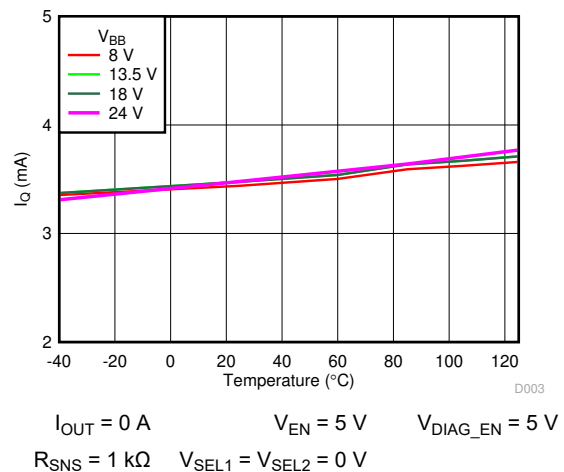
Figure 7-4. Quiescent Current ( I_Q ) vs Temperature
