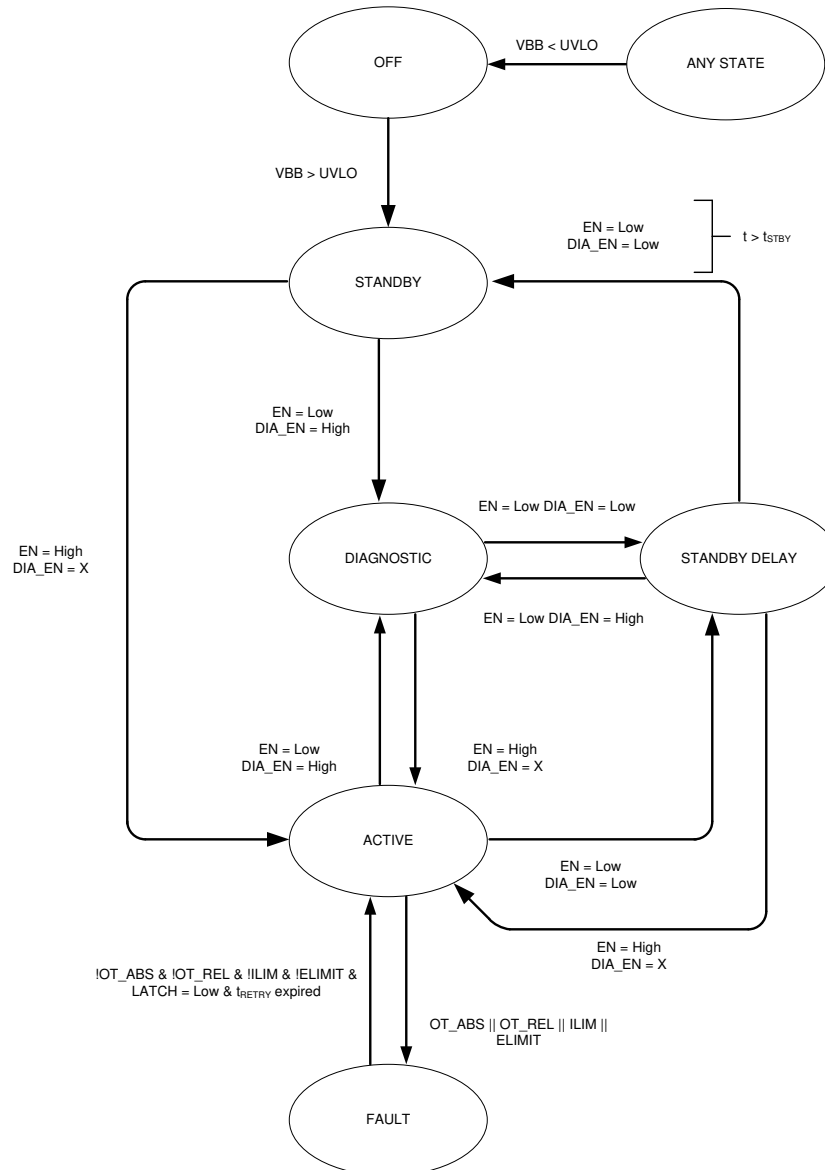
Figure 9-11. State Diagram
