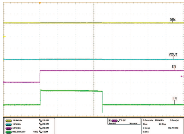
图 34. Output Hot Short to GND Response
