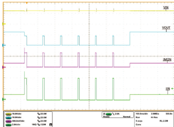
图 32. TPS2595x1, TPS2595x3, TPS2595x5 OverCurrent Response
