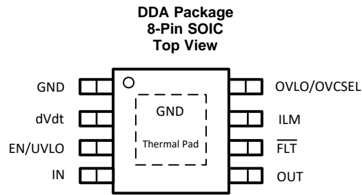
Pin Functions
